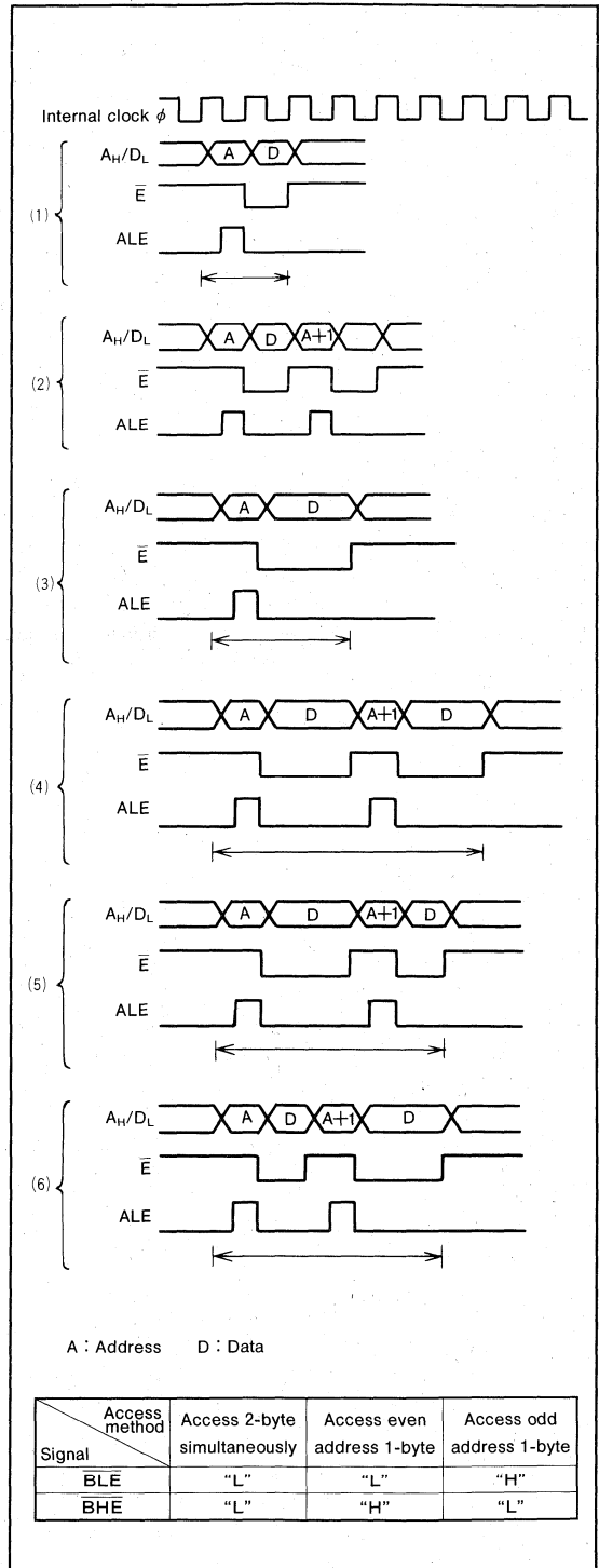
Fig.5 Relationship between access method and signals \bar{BLE} and B\bar{HE}
