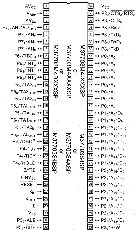
Outline 64P4B
