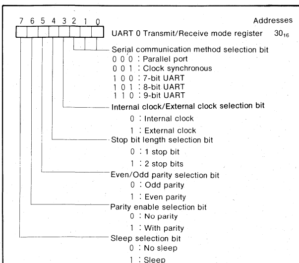
Fig. 39 UART 0 Transmit/Receive mode register bit configuration
