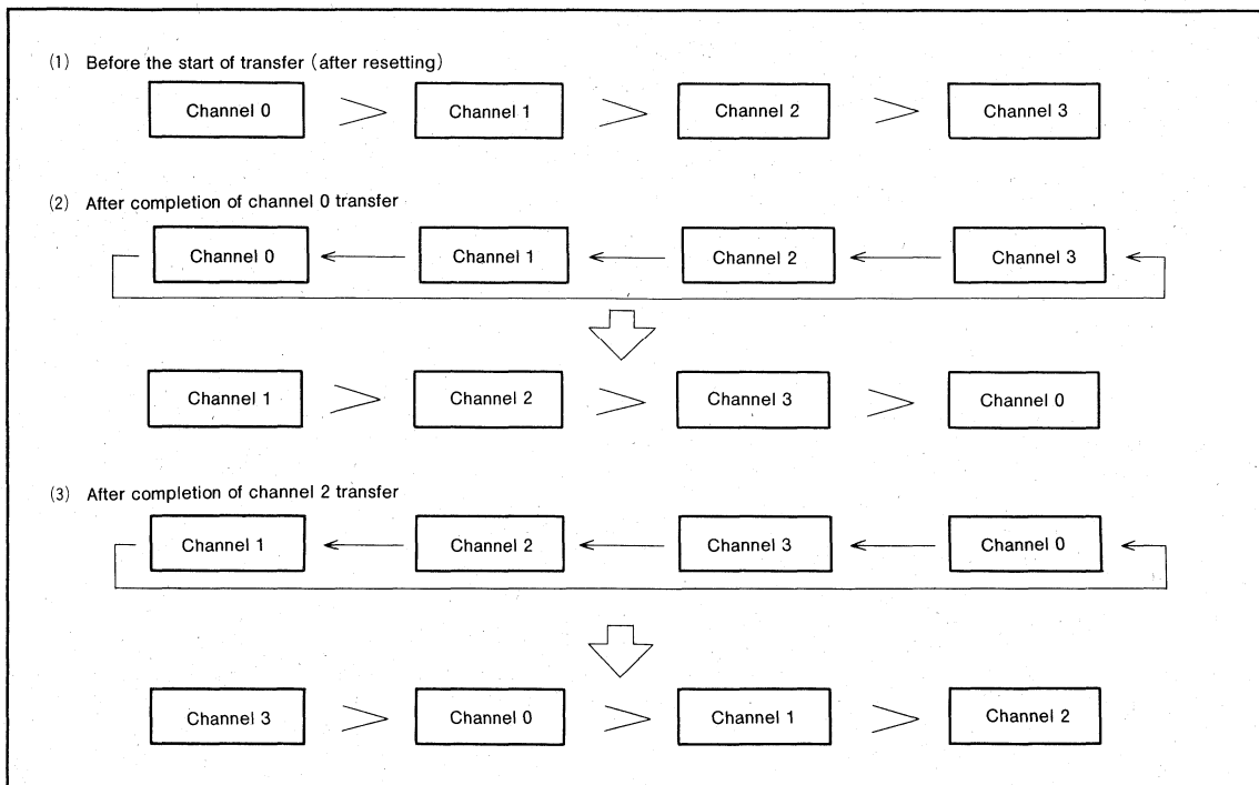
Fig.60 Rotative priority
