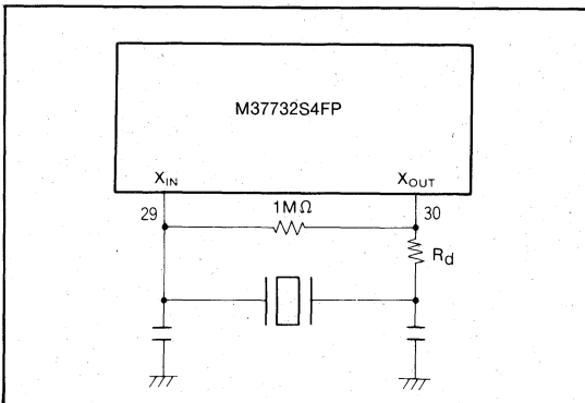
Fig. 61 Circuit using a ceramic resonator
