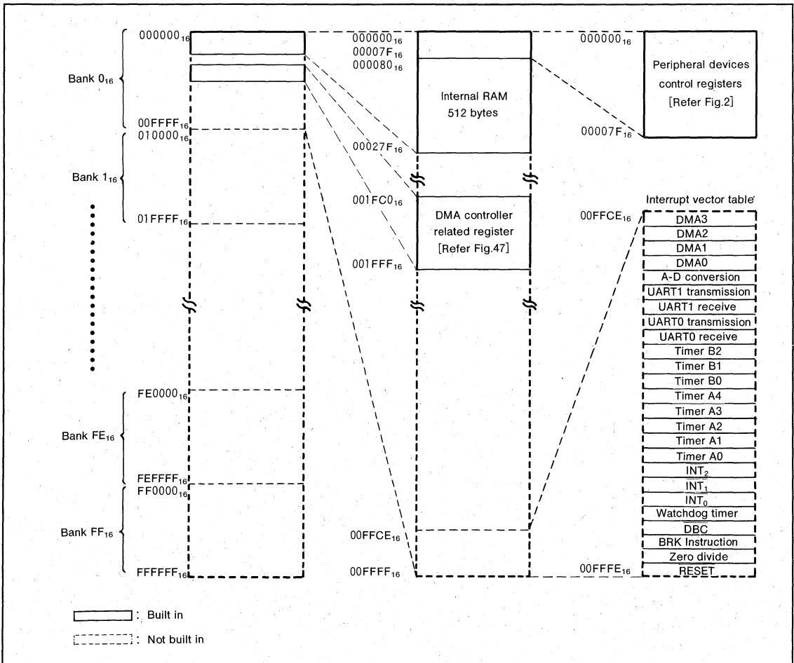
Fig.1 Memory map
