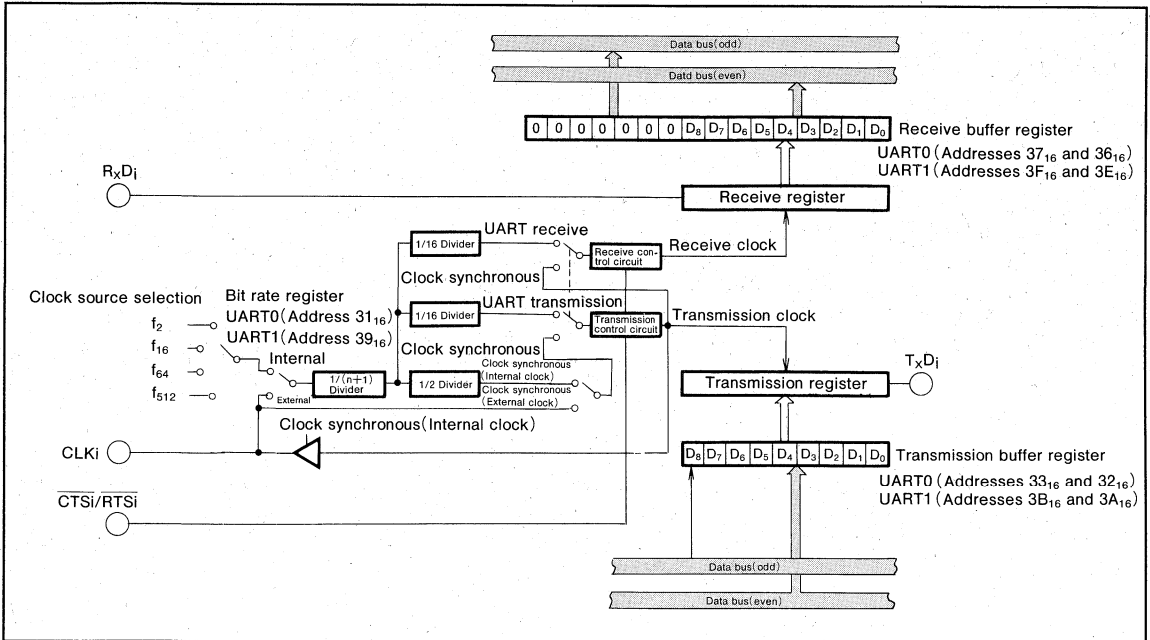
Fig.33 Serial I/O port block diagram
