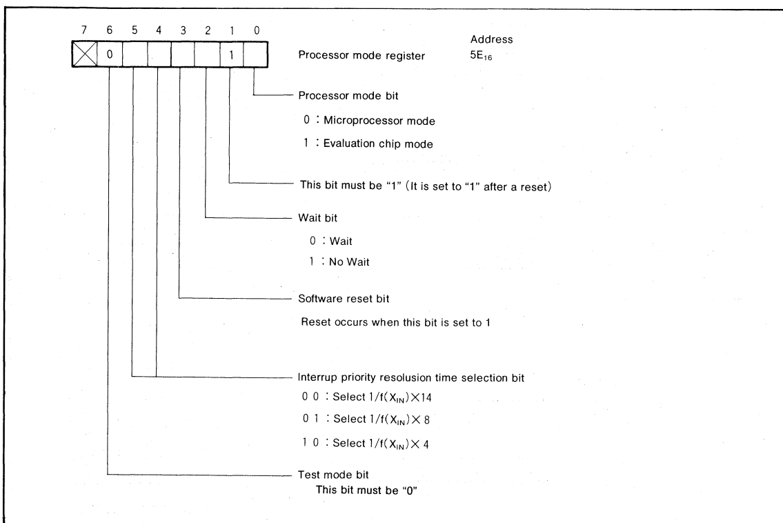
Fig. 53 Processor mode register bit configuration
