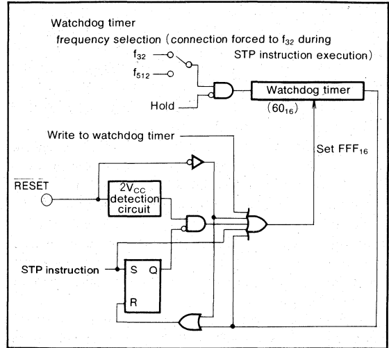
Fig. 48 Watchdog timer block diagram
