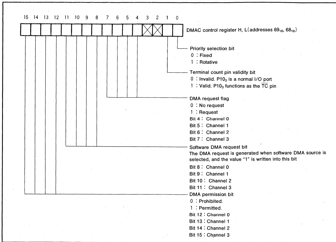
Fig.48 DMAC controll register bit configuration
