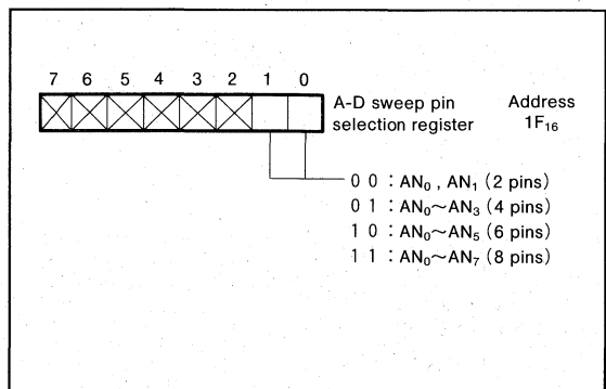
Fig.45. A-D sweep pin selection register configuration
