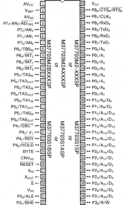
Outline 64P4B
