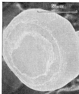
Fig.5 Lifted Au wire ball base
