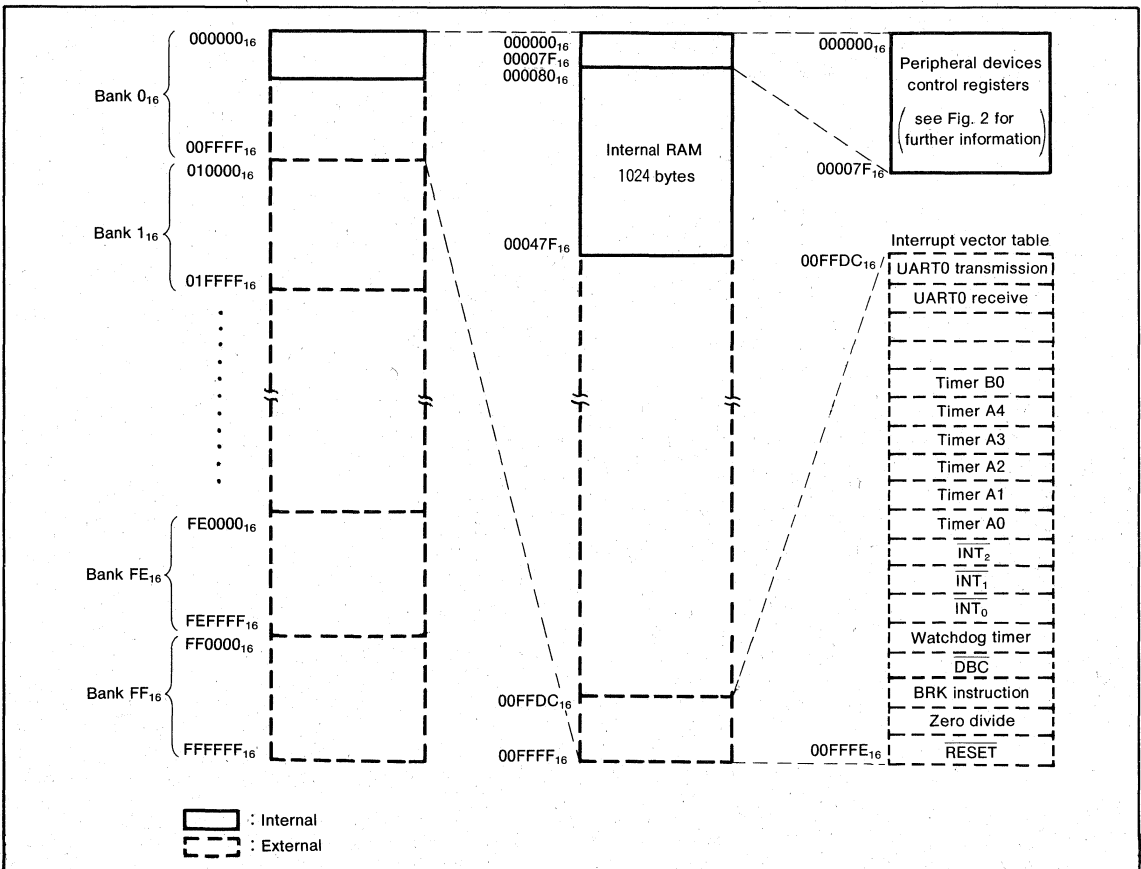
Fig. 1 Memory map
