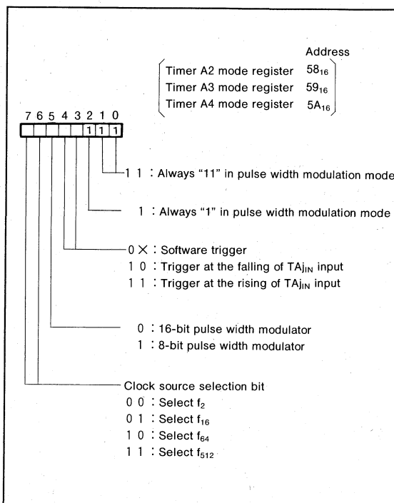
Fig.24 Timer Aj mode register bit configuration during pulse width modulation mode
