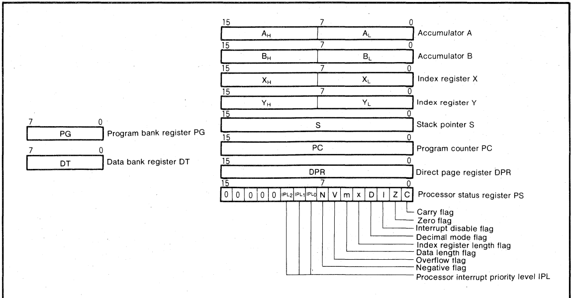
Fig. 3 Register structure
