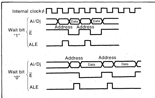
Fig. 59 Relationship between wait bit and access time
