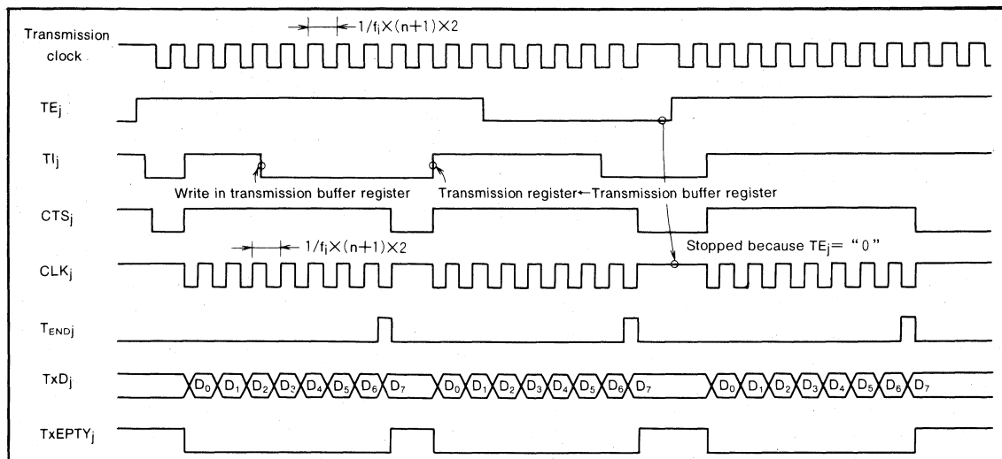
Fig. 39 Clock synchronous serial I/O timing
