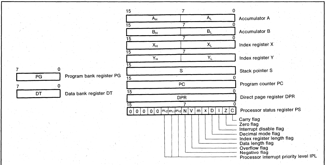
Fig.3 Register structure
