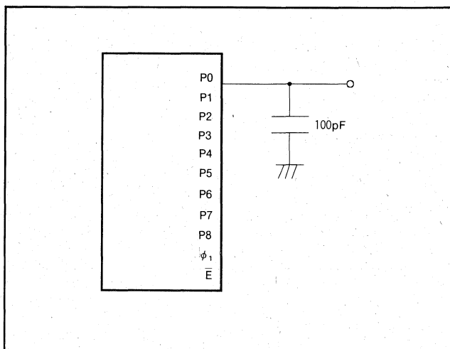
Fig. 1 Testing circuit for ports P0~P8, \phi_1
