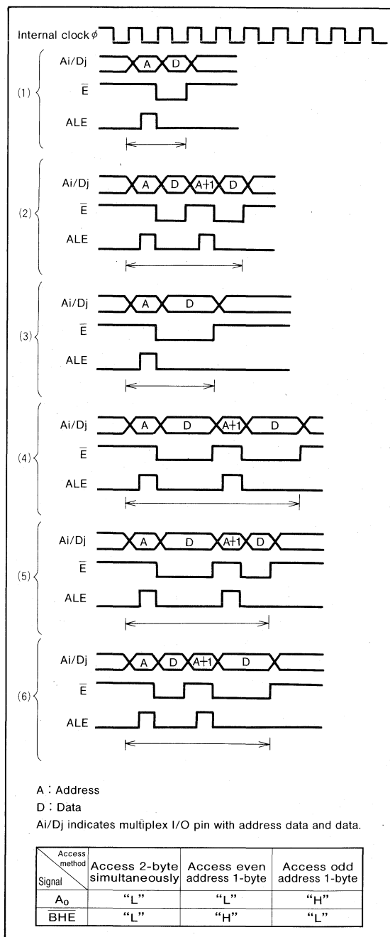
Fig. 5 Relationship between access method and signals A_0 and \overline{BHE}
