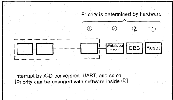
Fig.7 Interrupt priority
