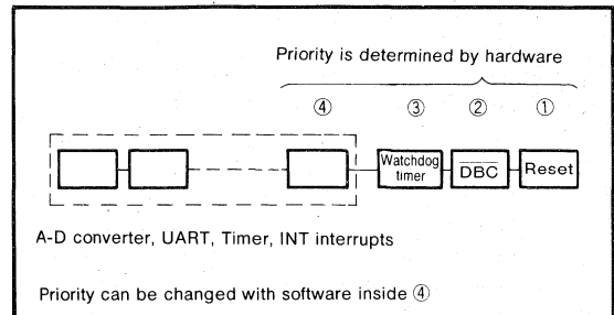
Fig. 7 Interrupt priority
