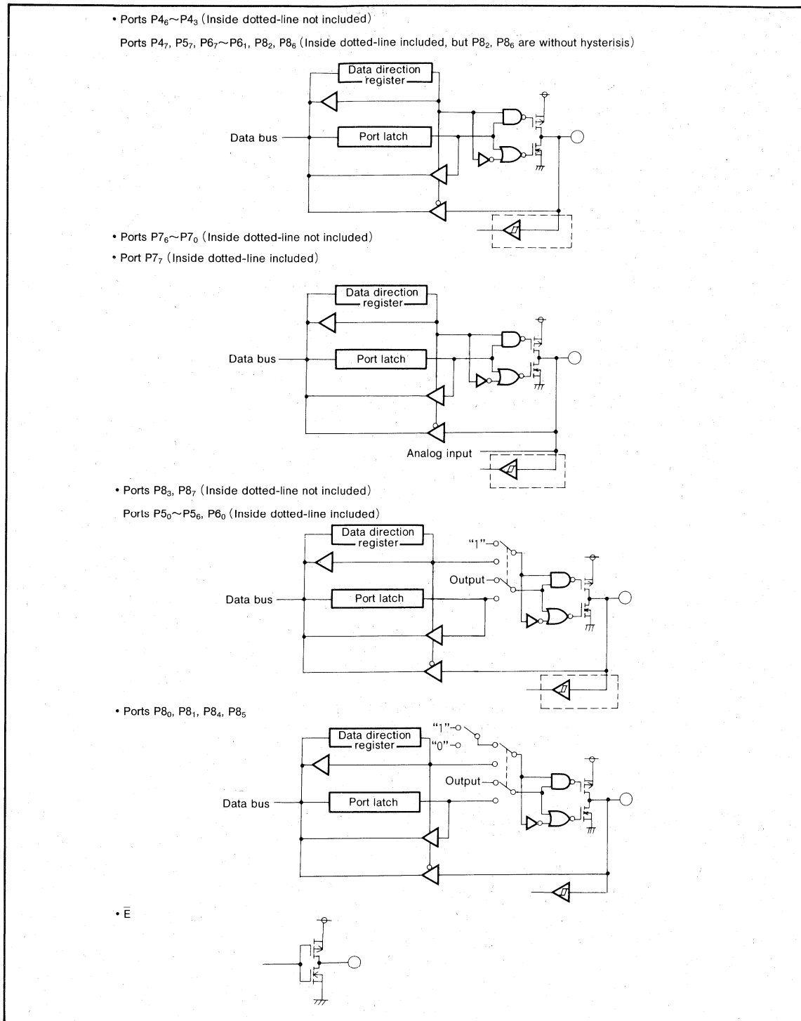
Fig. 55 Block diagram for ports P8 to P4 and the \bar{E} pin output
