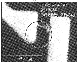
Fig.10 Aluminum trace of destructive spot
