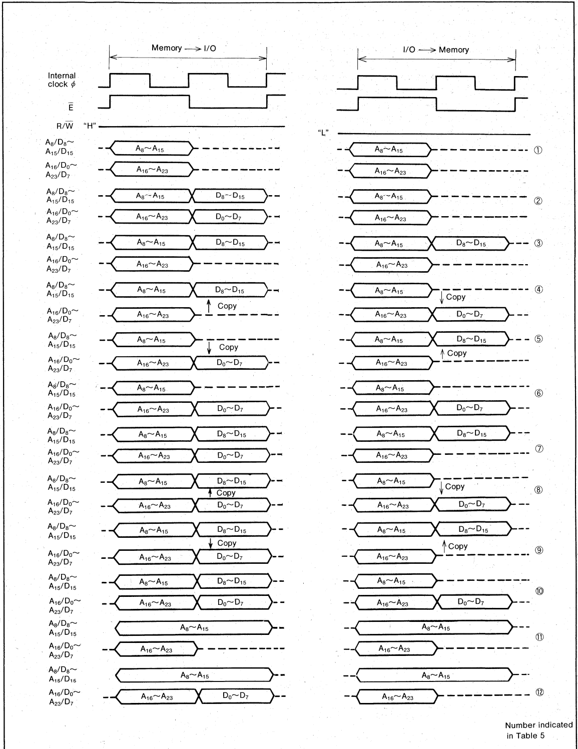
Fig.56 Data bus status under various conditions of one bus cycle DMA transfer
