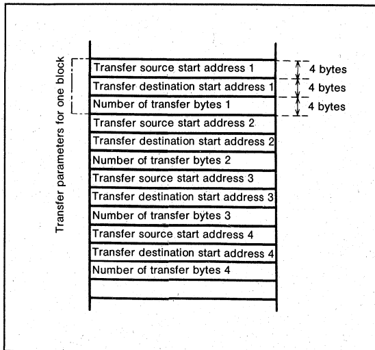
Fig.66 Array chain transfer mode parameter memory configuration example
