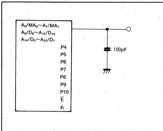
Fig.93 Testing circuit for ports
