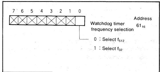
Fig. 49 Watchdog timer frequency selection flag
