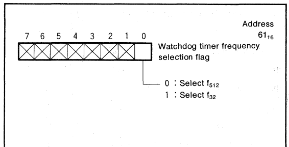
Fig.82 Watchdog timer frequency selection flag
