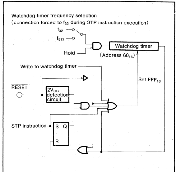
Fig.81 Watchdog timer block diagram
