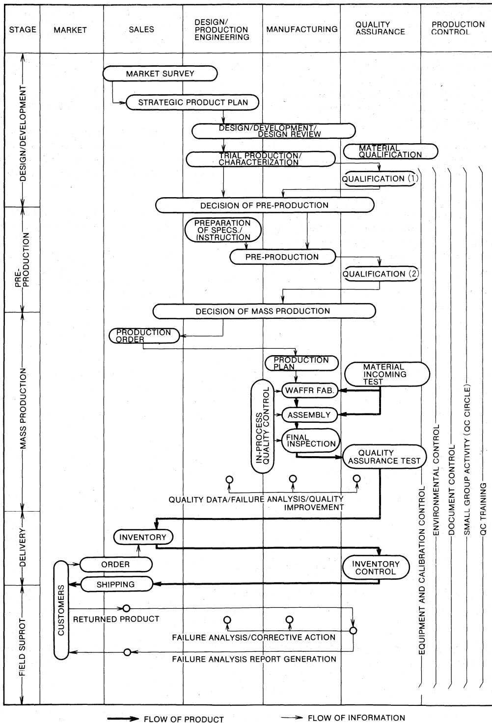
Fig.1 FLOW CHART OF QUALITY ASSURANCE SYSTEM
