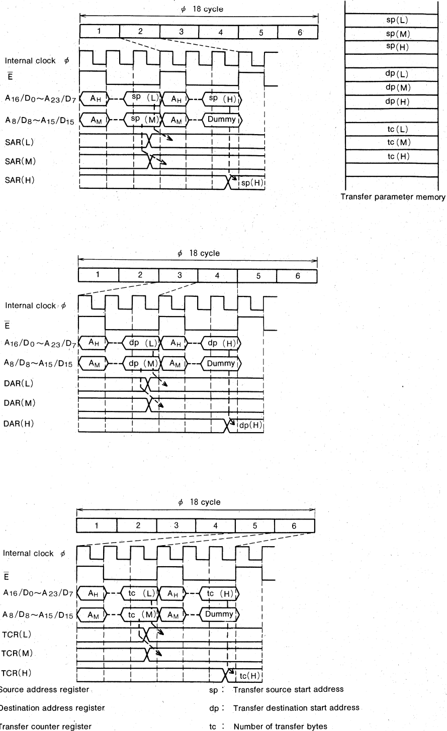
Fig.69 Array state example at 2 bus cycle transfer
