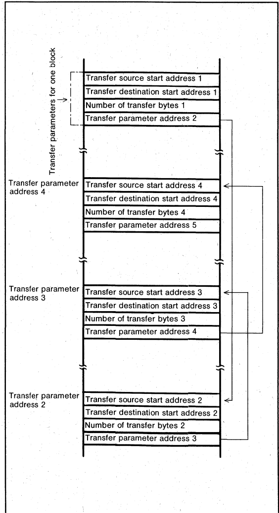
Fig.71 Link array chain transfer mode parameter memory configuration example
