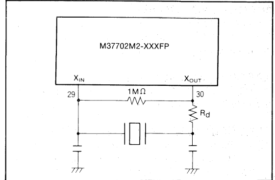
Fig. 56 Circuit using a ceramic resonator
