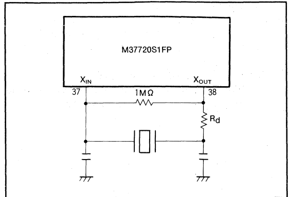
Fig.91 Circuit using a ceramic resonator
