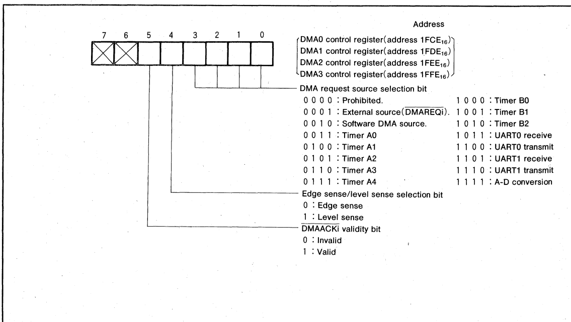
Fig.49 DMAi controll register bit configuration
