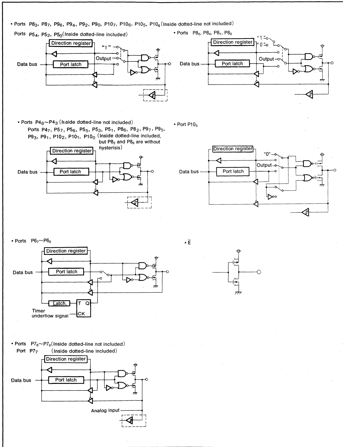
Fig.85 Block diagram for ports P10 to P4 in microprocessor mode and the \bar{E} pin output
